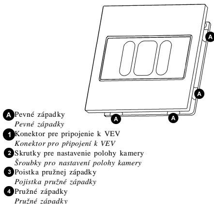
Obr. 3 Modul VEV0 4 FN 231 06/N2K, Modul VEV2 4 FN 231 07/N2K
